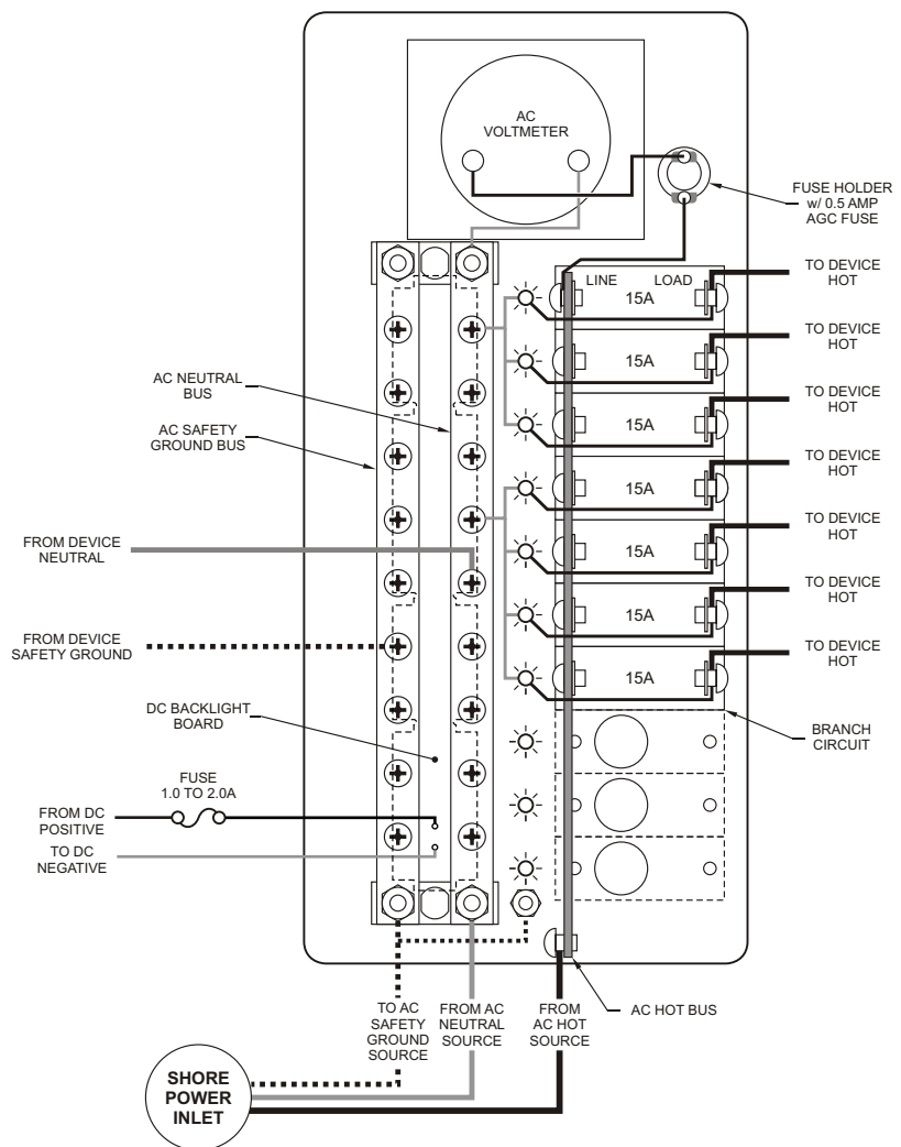
Wiring Diagram AC Power Distribution Panel with AC Voltmeter (Part Number 8478 / 3478 shown for reference)
