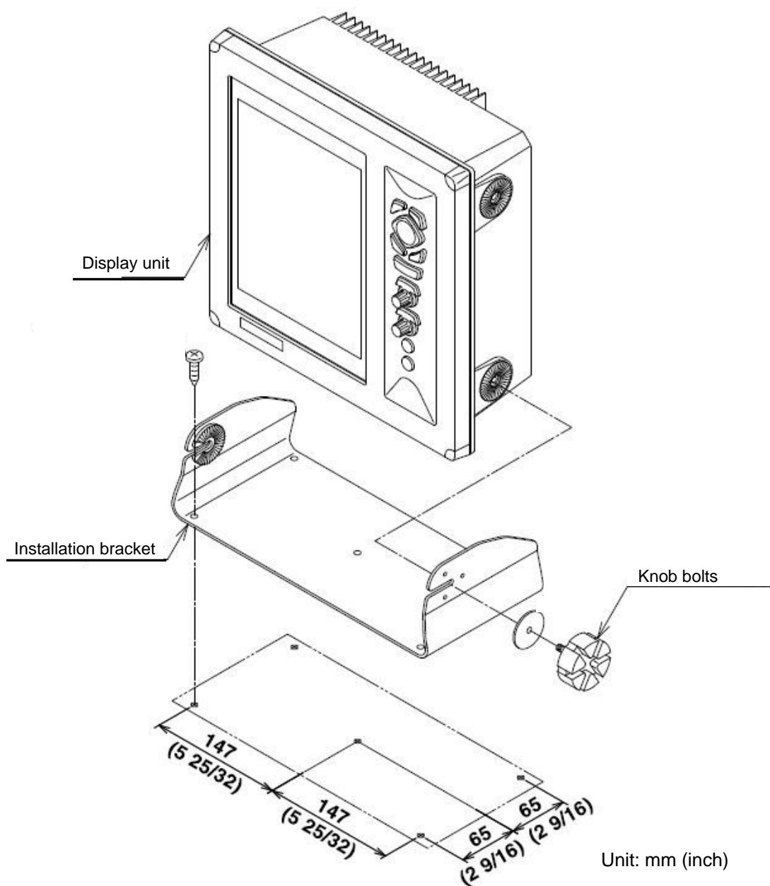
Fig. 5.2 Desk-top installation
