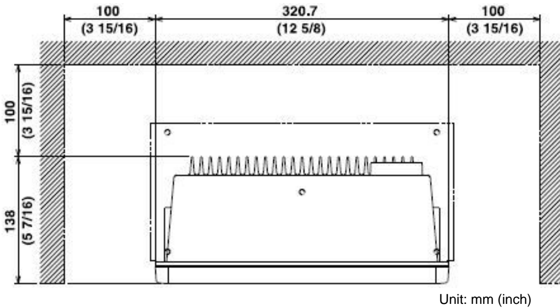
Fig. 5.3 Maintenance space
