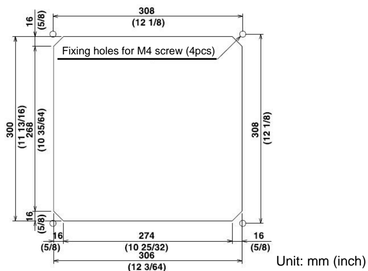
Fig. 5.5 Work of flush-mount installation hole
