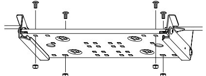
Dual mount applications 4 Carriage bolts & lock nuts. Only 4 bolts required for grill mounting. Place bolts (2 per side) diagonally from each other as shown.
