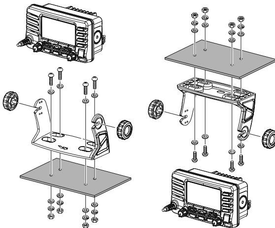
DESKTOP MOUNTING
