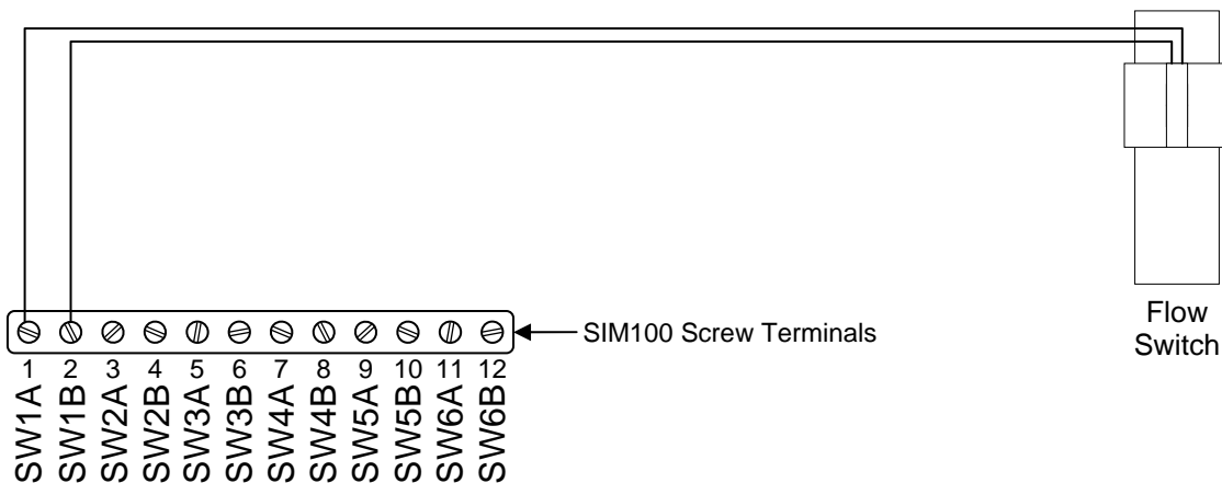
Figure 1 - Wiring Diagram
