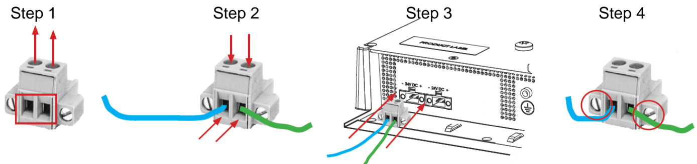
Figure 9 – Attaching Power Cables to Connector
