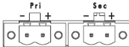
Figure 8 – Power Connections
