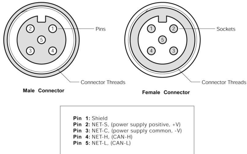
Figure 10 – NMEA 2000 ® Connector Face Views
