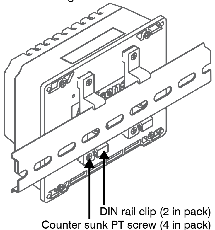
Figure 2 - Mounting Options
