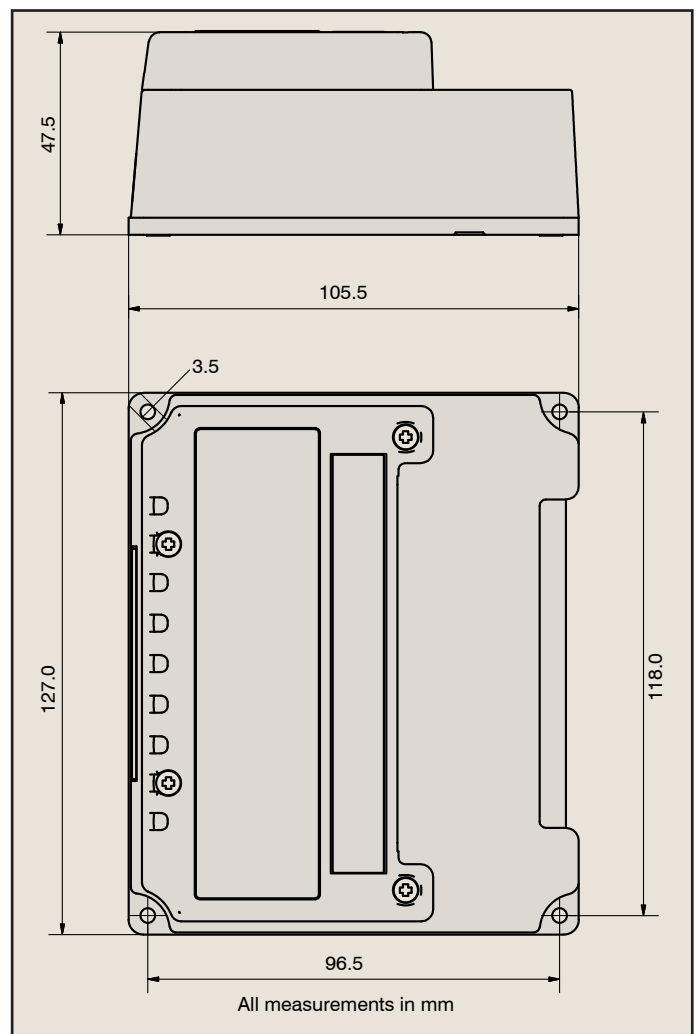
Figure 8 - Dimension Diagram
