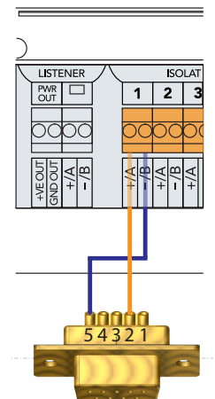
Figure 7 - RS232 Listener Connection
