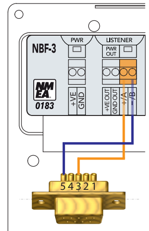
Figure 5 - RS232 Talker Connection
