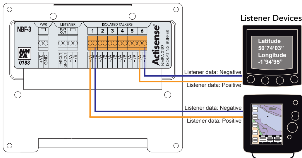
Figure 6 - Talker Port Wiring Diagram
