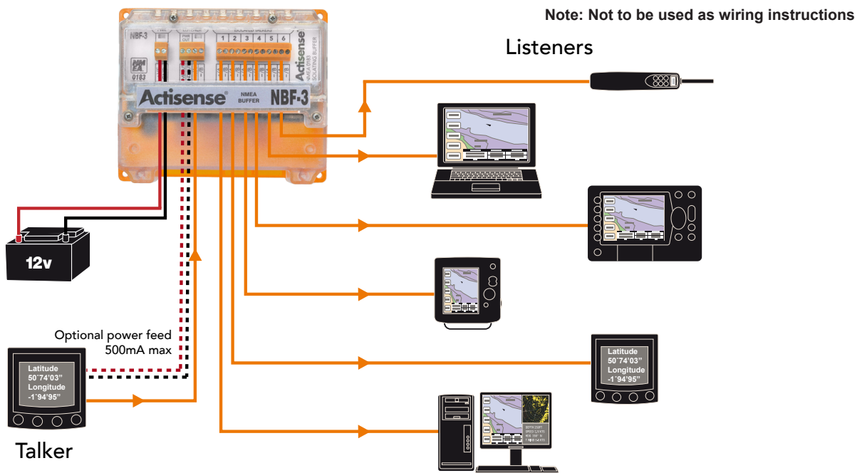
Figure 1 - Example of a Typical NBF-3 Installation
