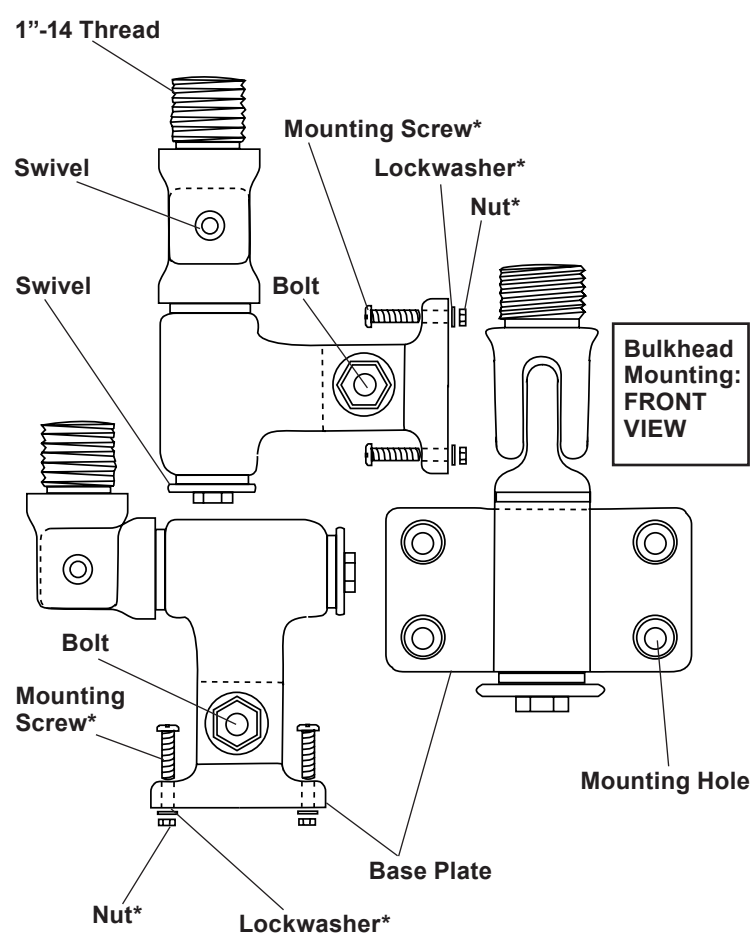
Deck Mounting: SIDE VIEW
