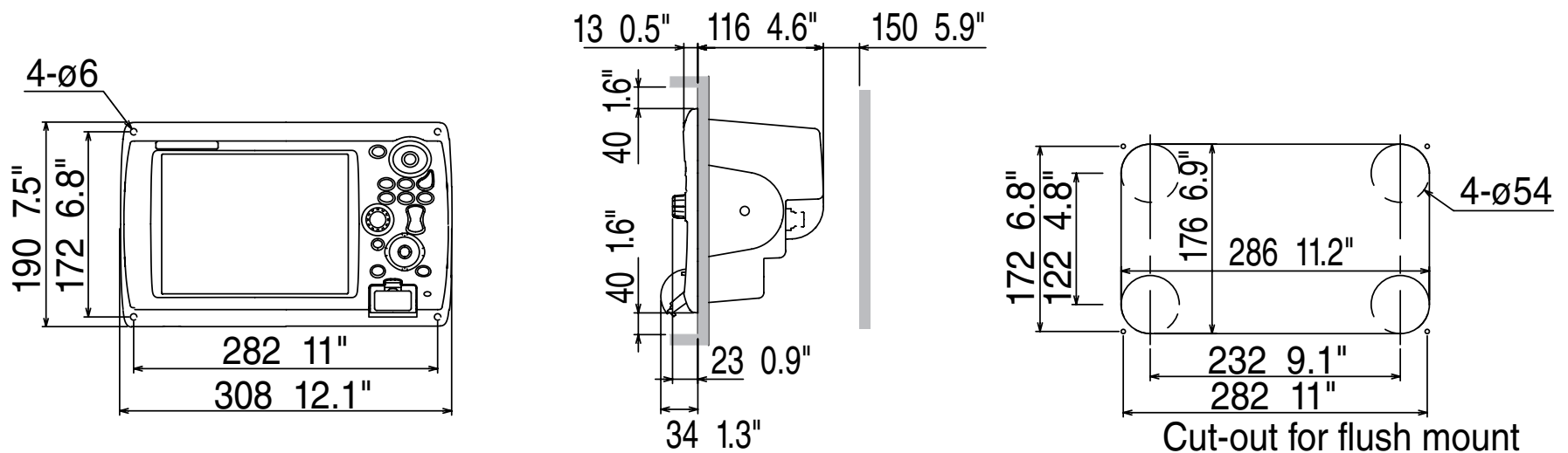
Multi Function Display (Flush Mount) MFD8
