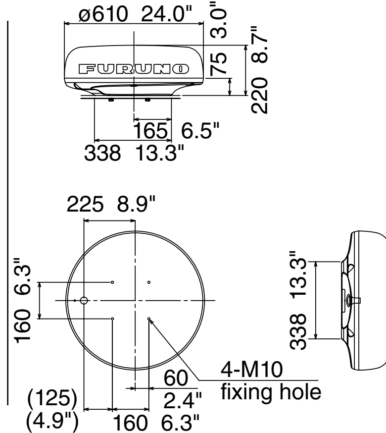
24" Radome Radar Sensor DRS4D 7.5 kg 16.5 lb
