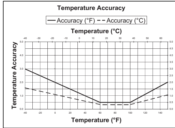
Figure 1. Temperature Accuracy
