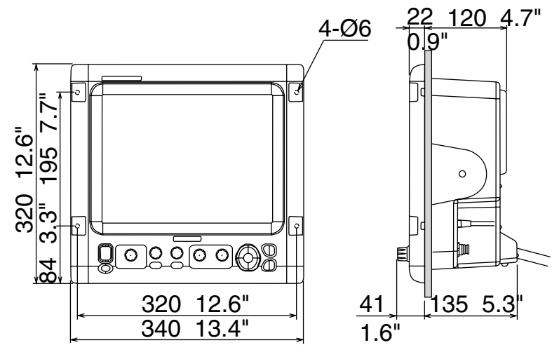
FCV1150 (Flush Mount)
