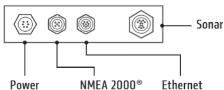
Control Head Ports
