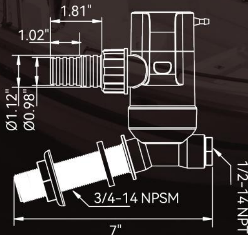
Split quick-connect joint design no need to disconnect base or plumbing when replacing pump.
