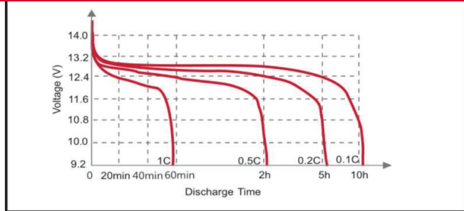
DIFFERENT RATE DISCHARGE CURVE (25°C)
