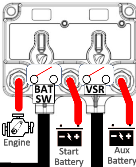
Fig 13 - Dual XD - 86 Series (DTM Connectors) (Matches Legacy Remote Relay Solutions)
