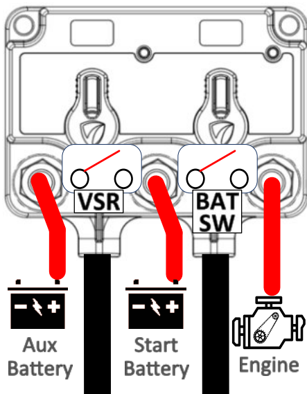
Fig 12 - Dual XD - 85 Series (Flying Wires)
