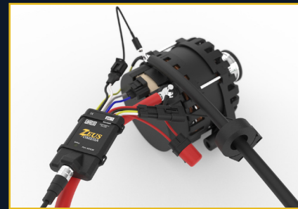
ADM with Pre-Terminated wires connects to the alternator.
