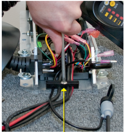
FIGURE 31 Reinstall strain relief screw.
