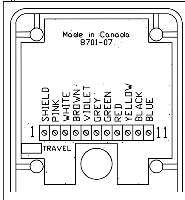
Figure 2 - Remote Cable Connections
