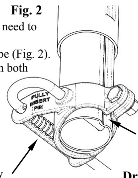
Plunger pin assembly
