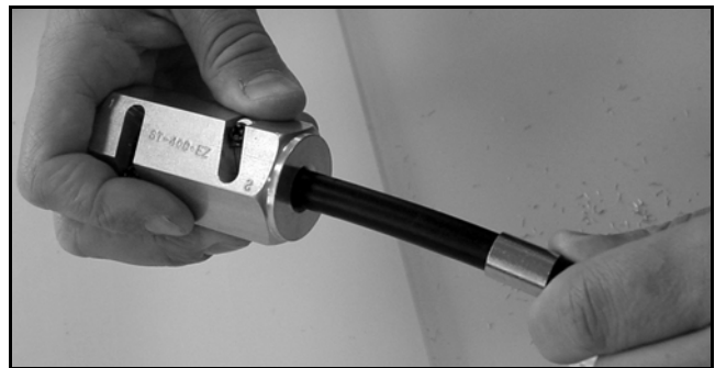
Figure 84: Stripping the Cable Jacket
