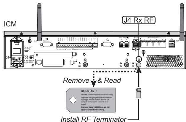
Figure 28: RF Terminator and Instructions Tag
