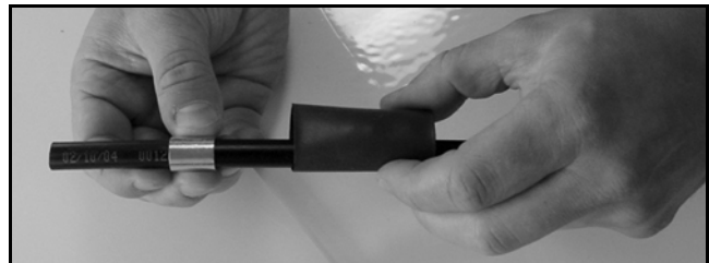
Figure 81: Placing the Heat Shrink Tubing and Ferrule
