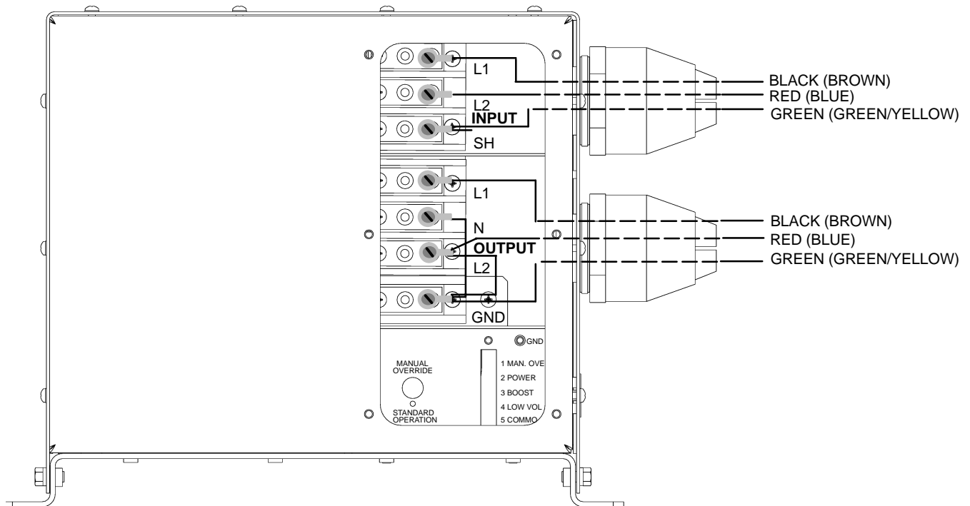
Figure 8. Typical Wiring for European 3-Wire, single-phase 230 Volt
