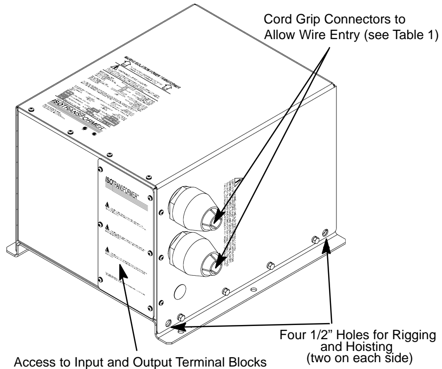
Figure 4. IsoTransformer Access Openings
