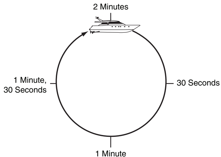
Figure D-3 Timing the Calibration Circle
