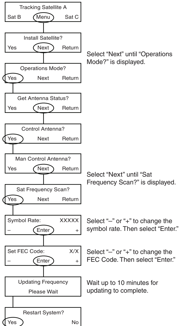
Figure A-2 Scanning Frequency Data
