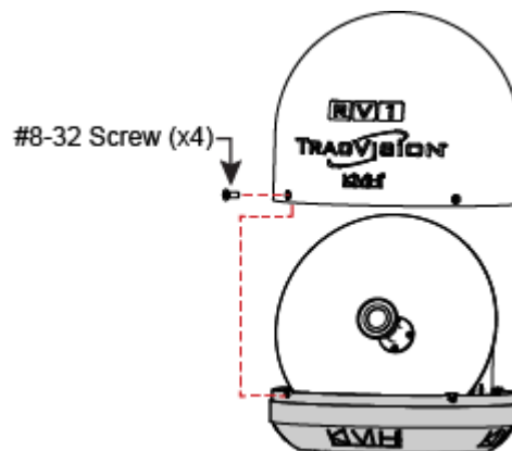
Figure 4-1 Radome Removal
